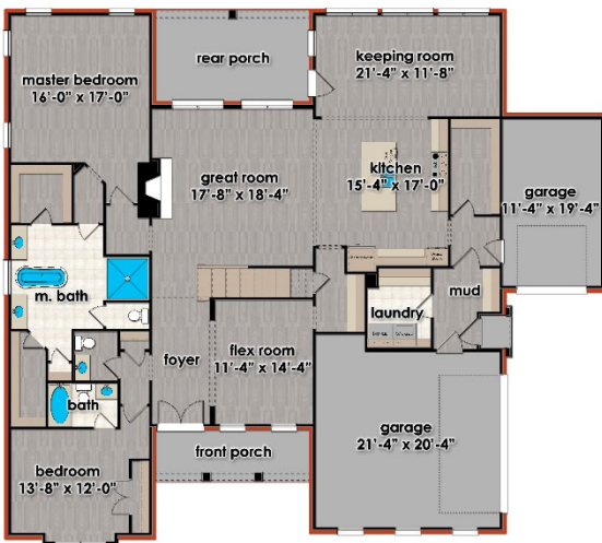
Main Level Floor 2,648 sf
