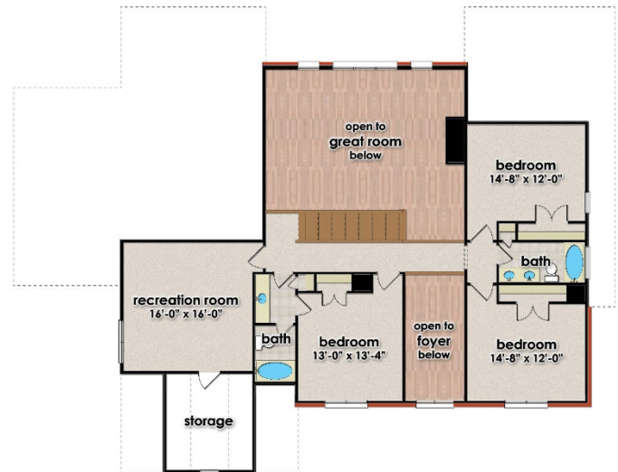
Upper Level Floor 1,231 sf
