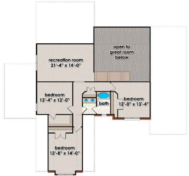
Upper Level Floor 1,167 sf
