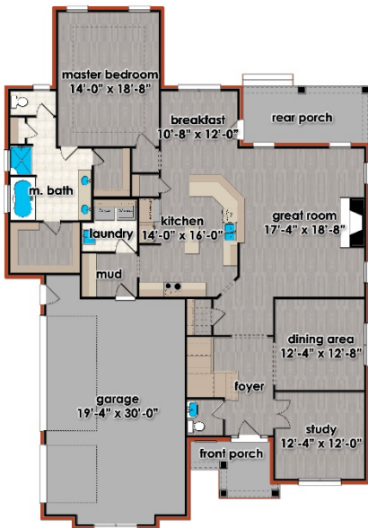
Main Level Floor 2,101 sf
