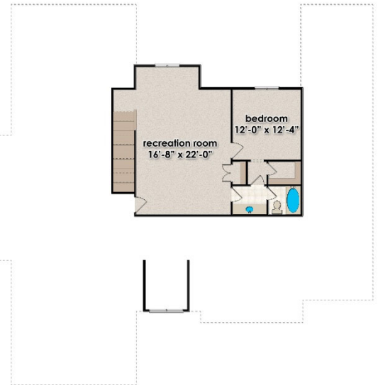
Upper Level Floor 719 sf
