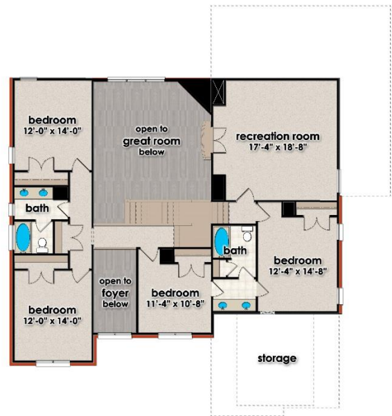
Upper Level Floor 1,560 sf
