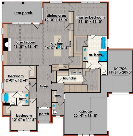
Main Level Floor 2385 sf
